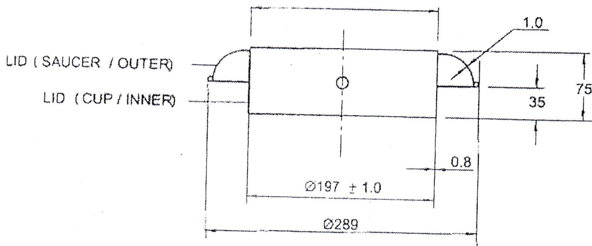
FIG 2 LID FOR STAINLESS STEEL MILK CAN — TRANSPORT TYPE (20, 30, 40 AND 50 LITRE)
